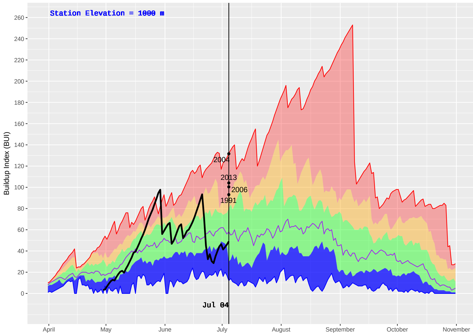
SUCCOUR CREEK (374) : Historical (1986–2016) and Current (2018) Noon Buildup Index (BUI)
