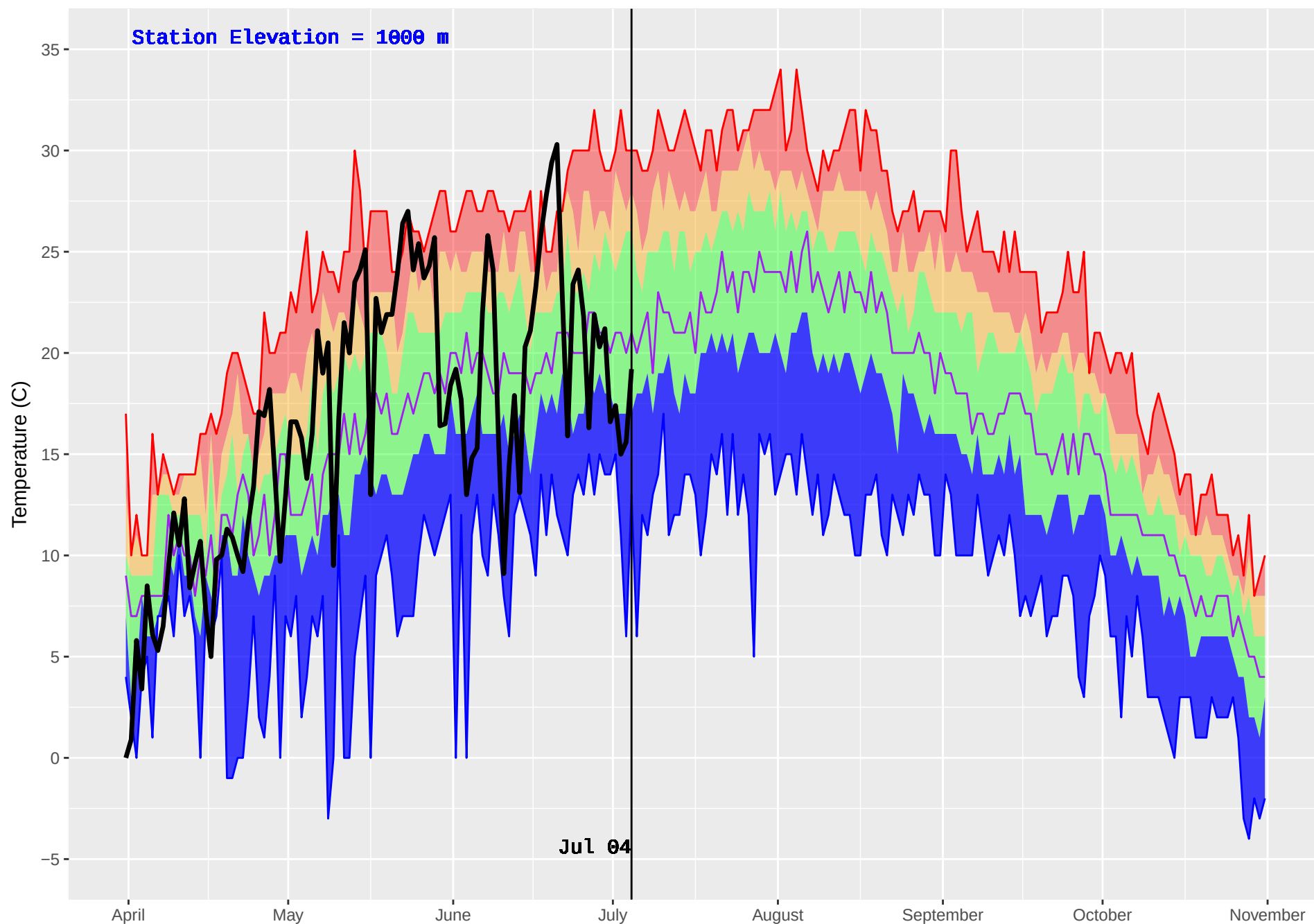
SUCCOUR CREEK (374) : Historical (1986–2016) and Current (2018) Noon Temperature
